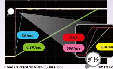
CC Mode: 0-120A (PXZ20K-500)
